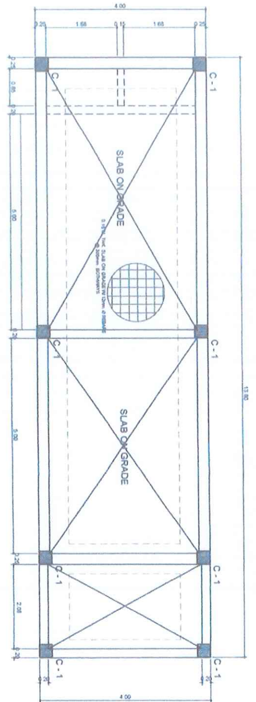
FOUNDATION PLAN
