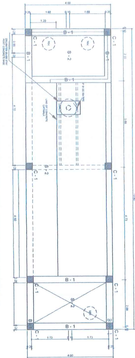
CONCRETE COVER SLAB STRUCTURAL LAY-OUT PLAN
